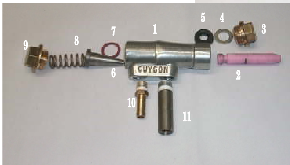
Exploded View of Blast Gun
